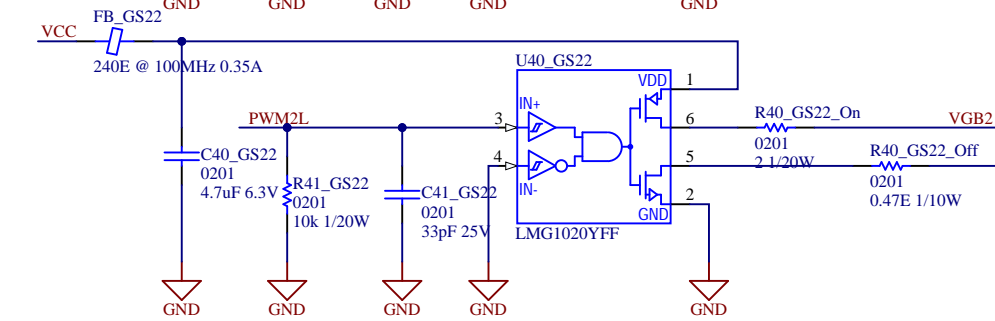
Secondary-side Gate Drivers
